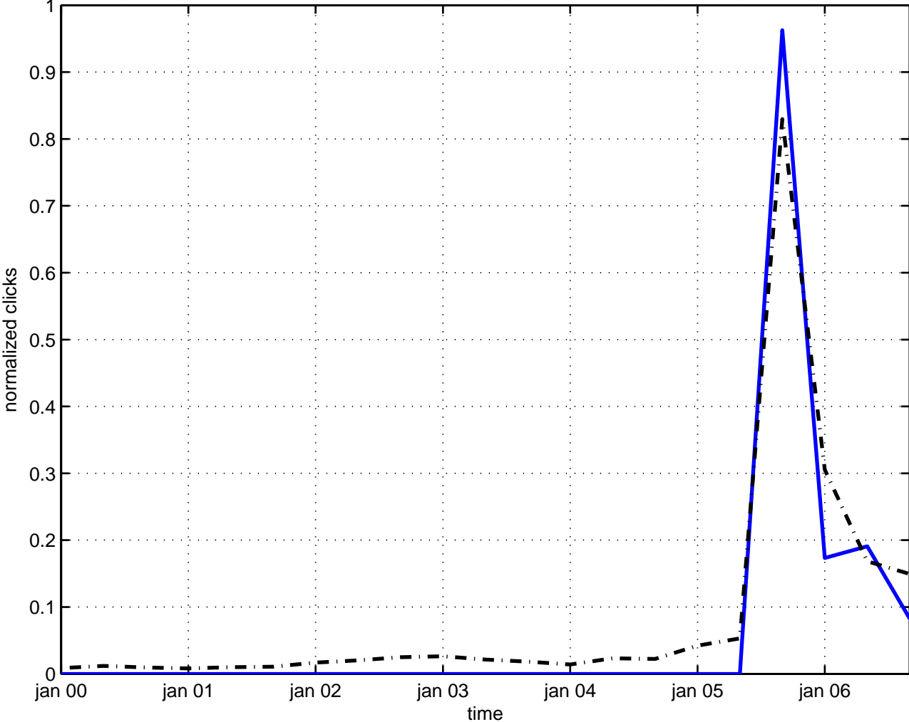
heterotic cosmic string
