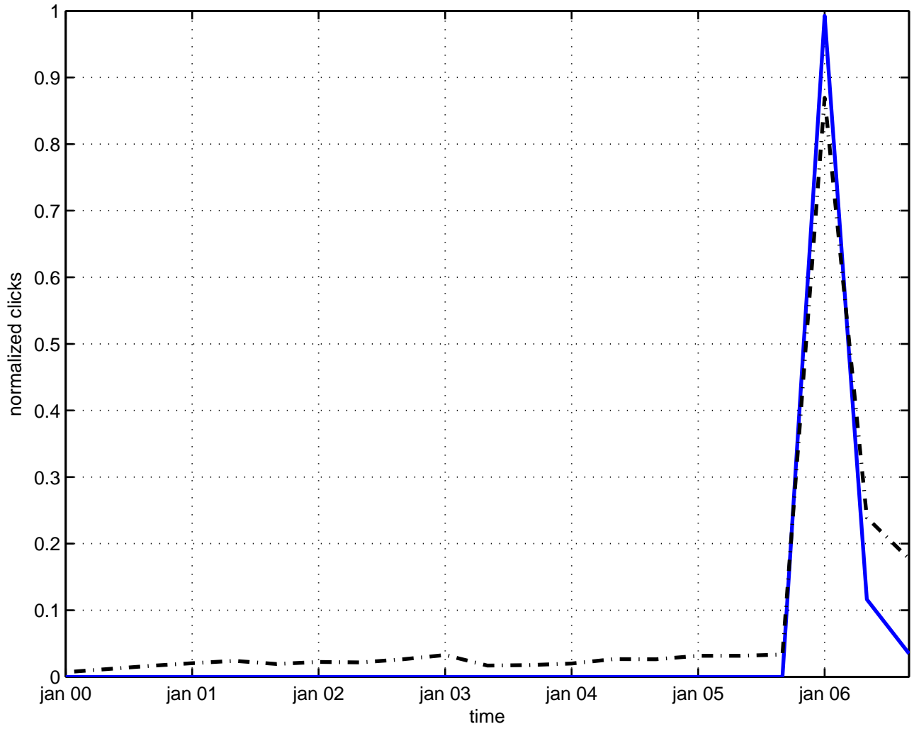
hessence dark energy
