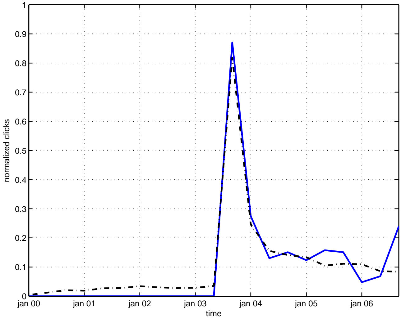
helicity photon
