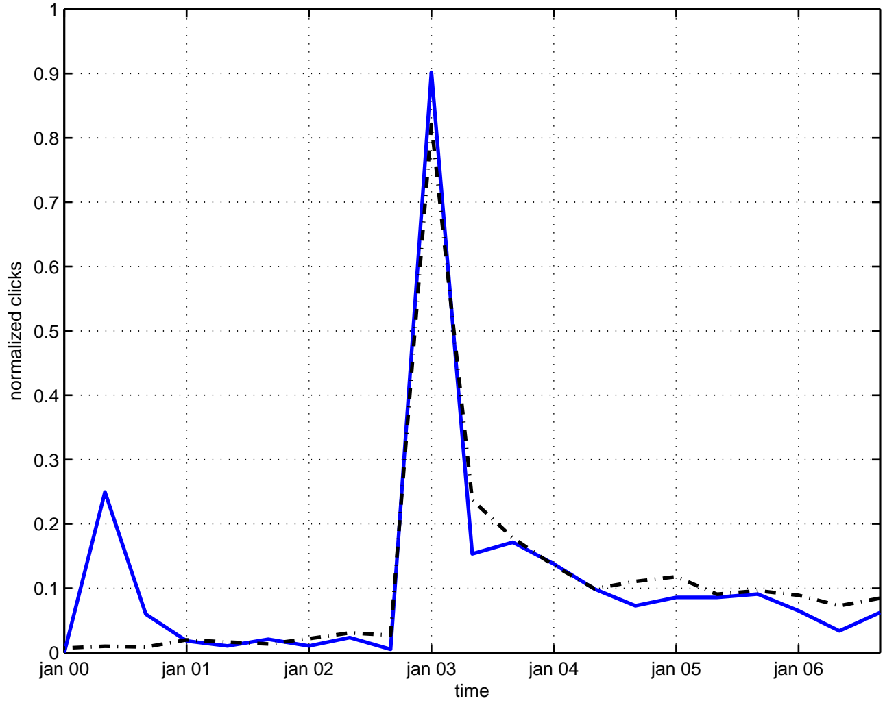
heisenberg field equations
