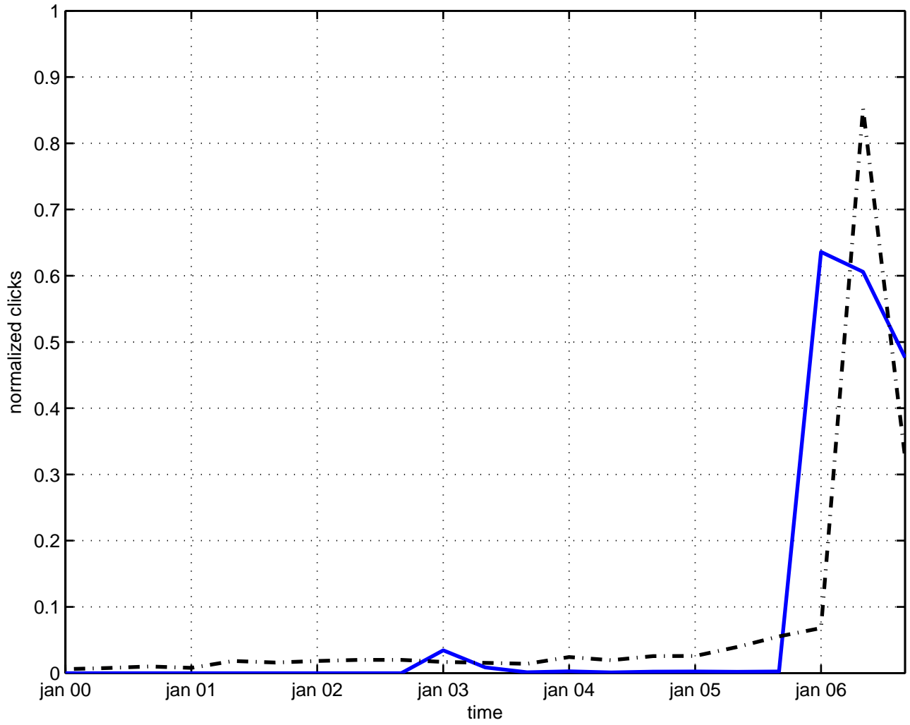
hecke operator
