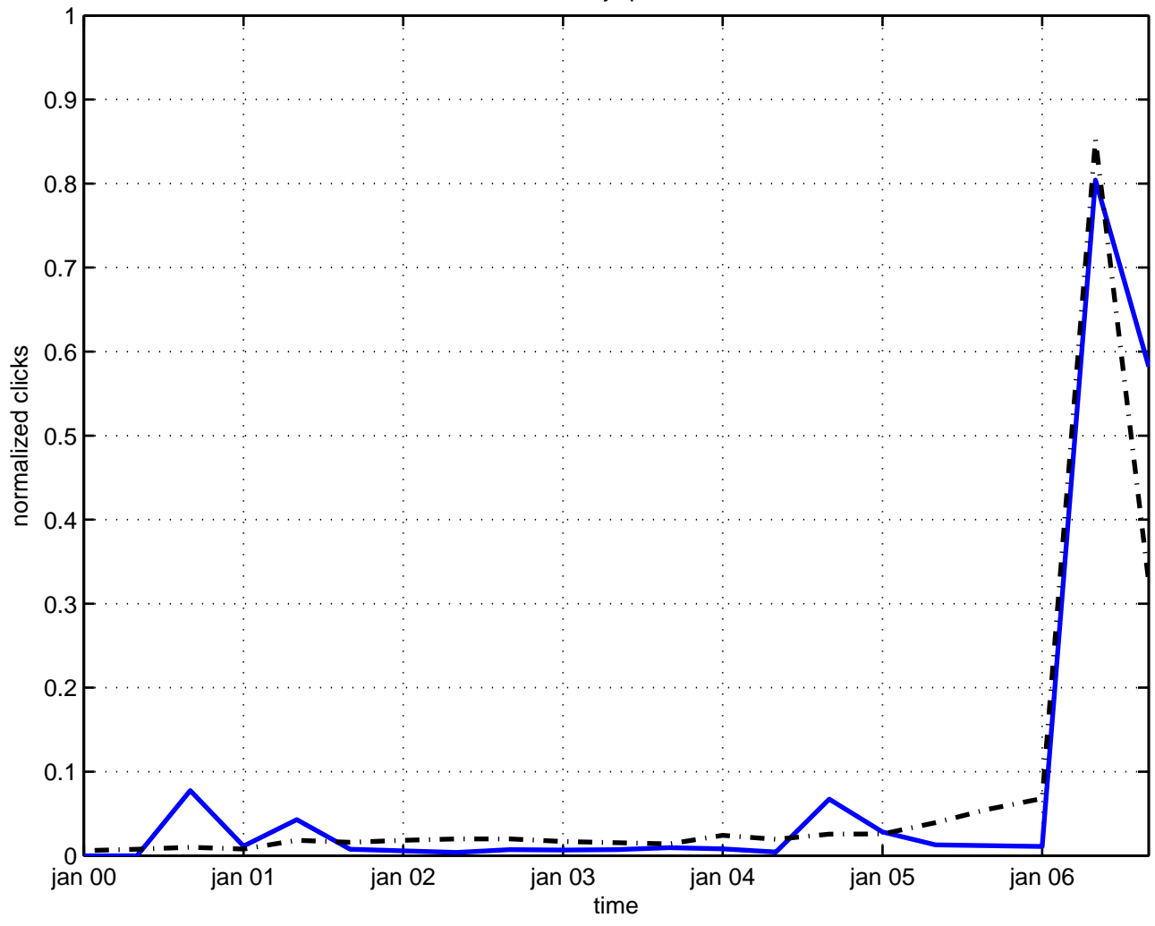
heavy quark
