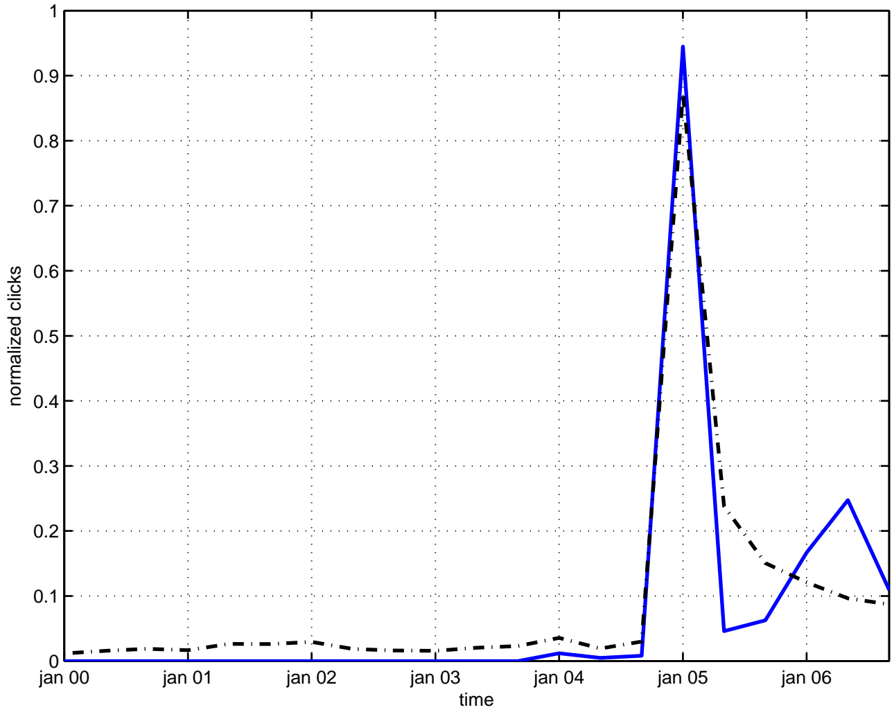
heavy ion scattering
