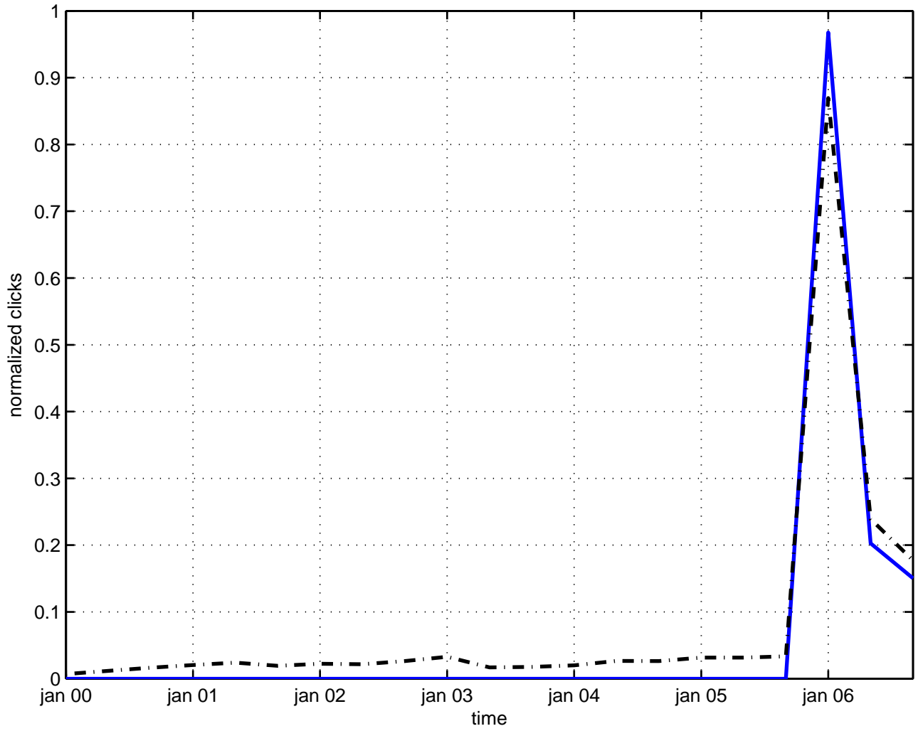
heavy hadron
