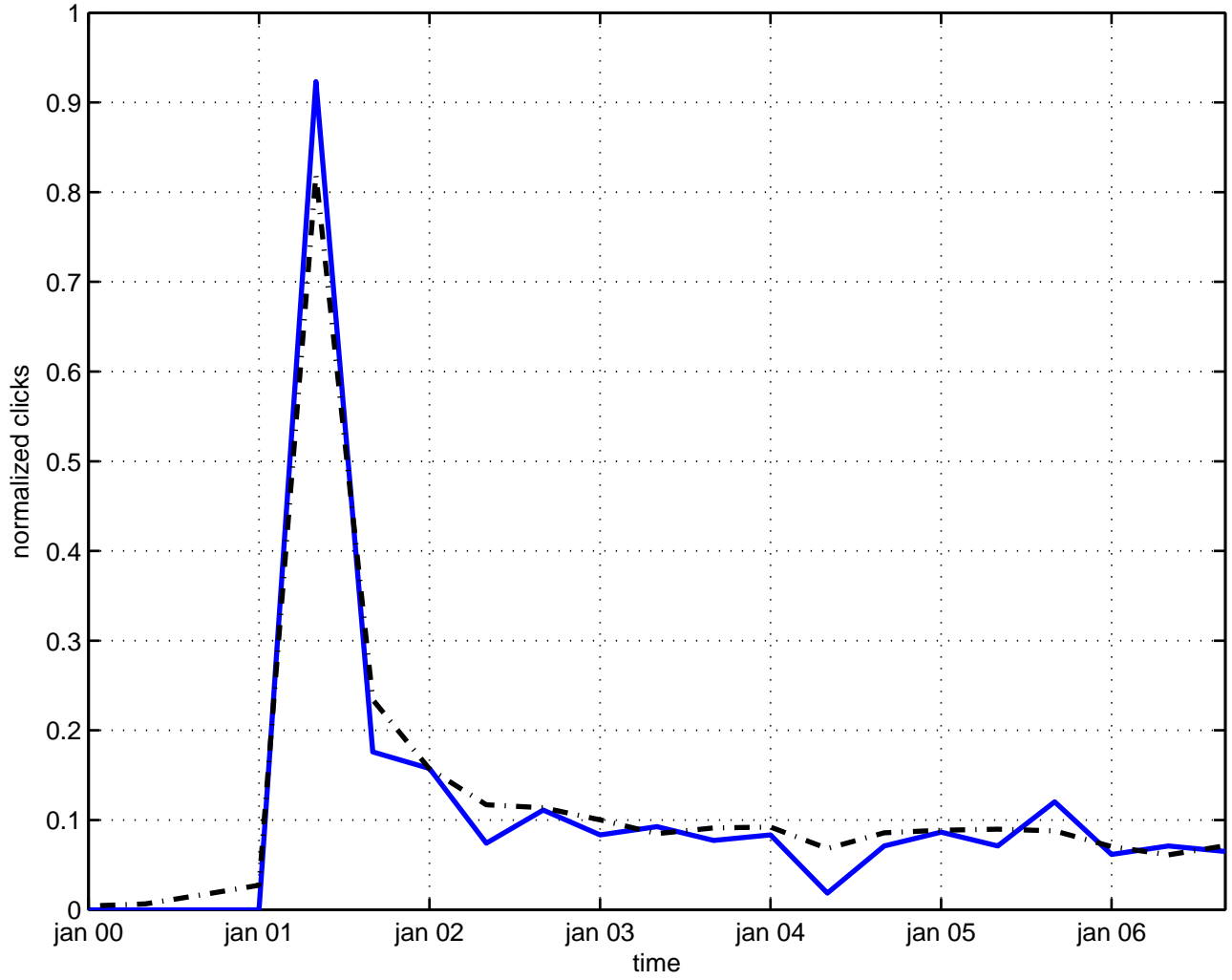
heat kernel operator
