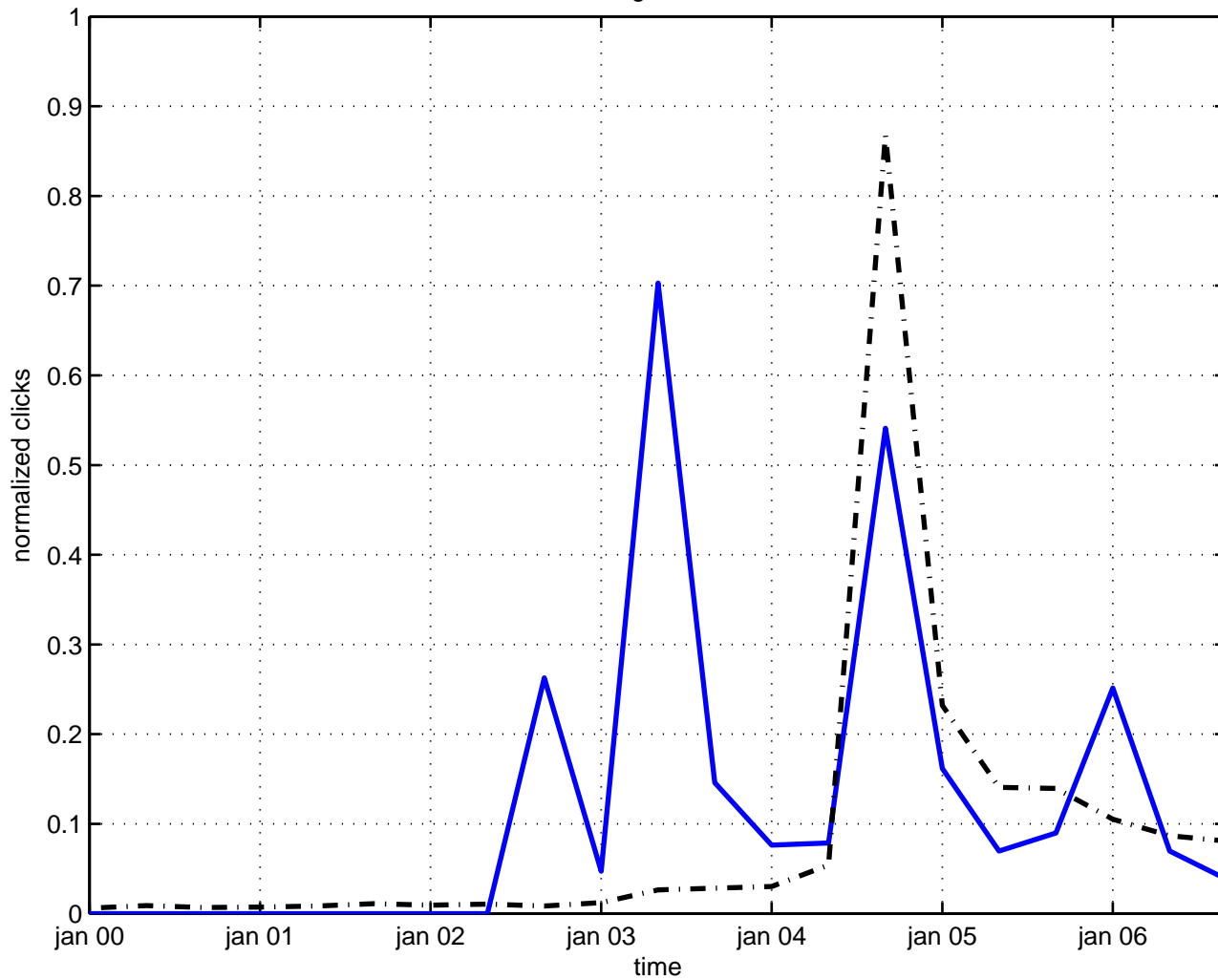
hawking wormhole
