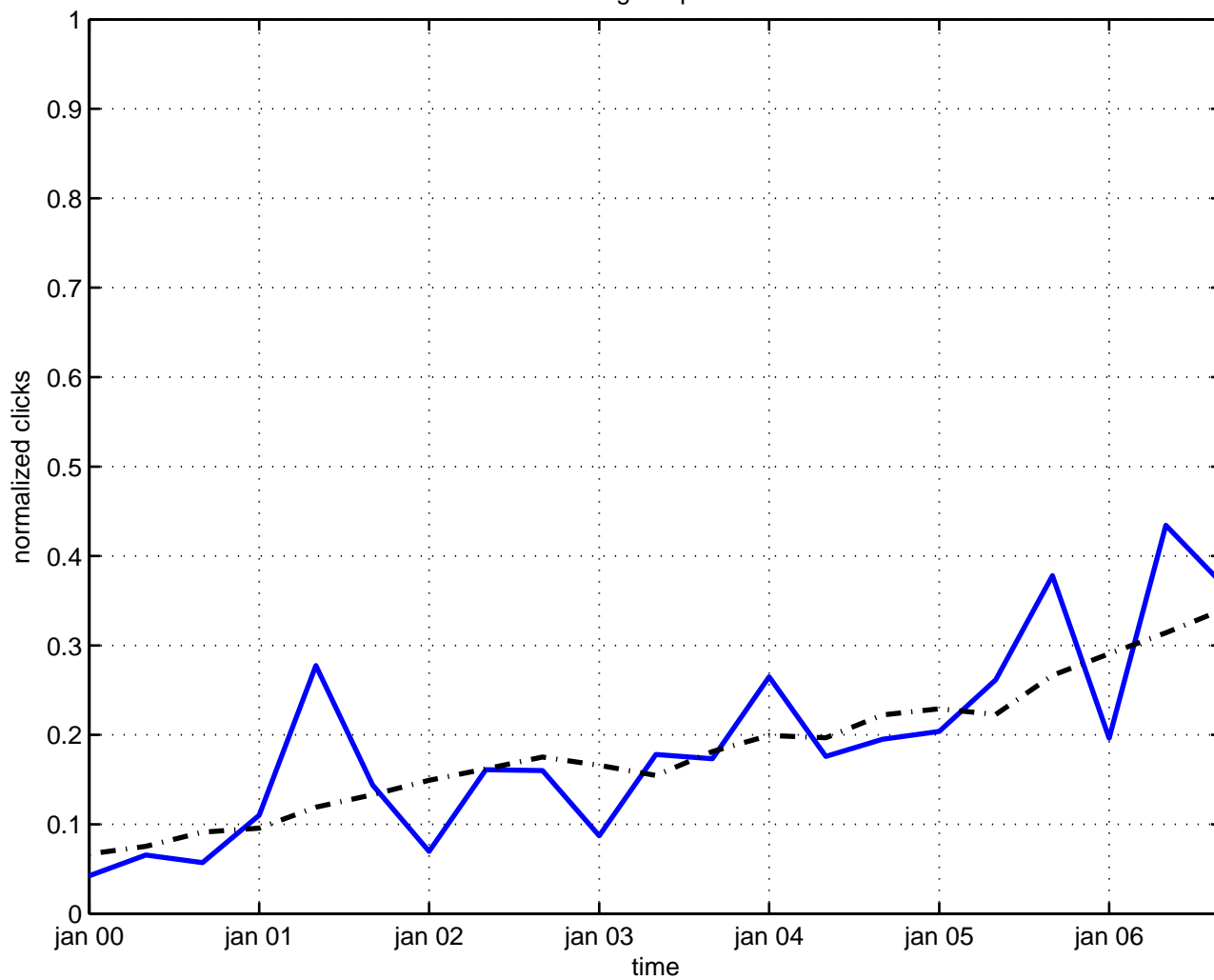
hawking temperature
