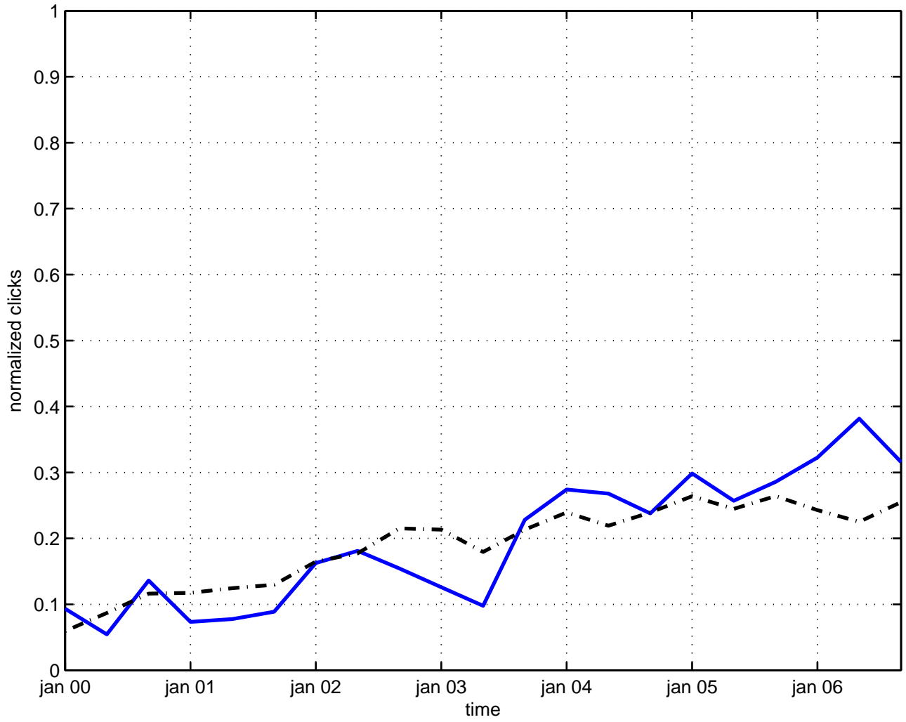
hawking radiation
