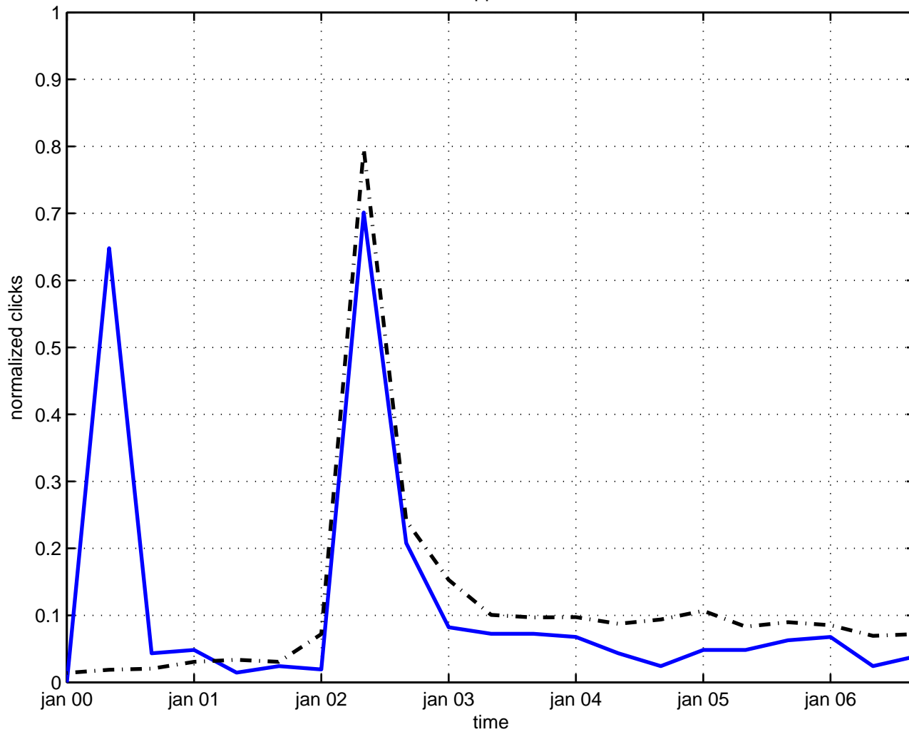
hartree approximation
