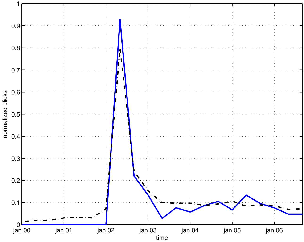
harmonic space
