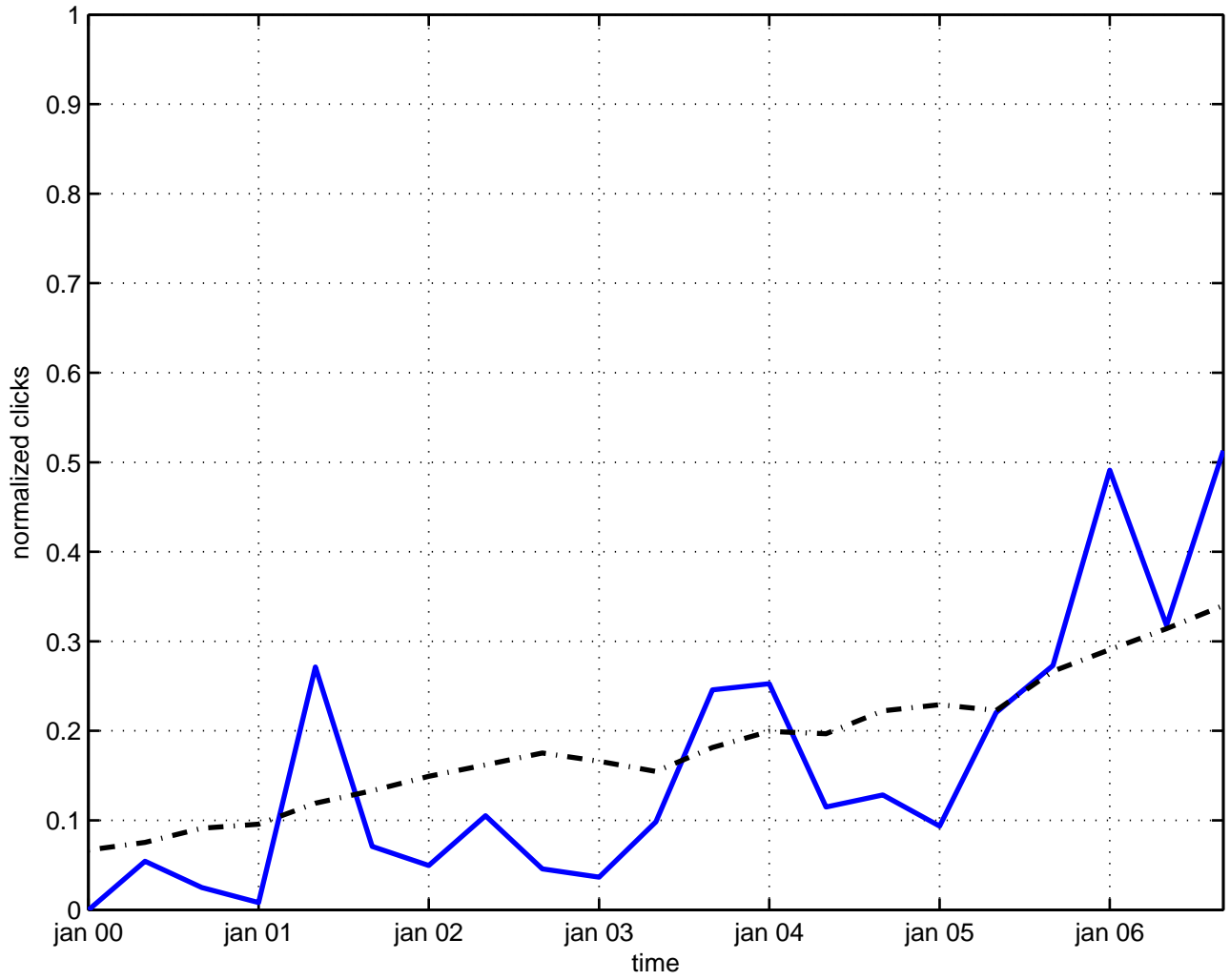
harmonic expansion
