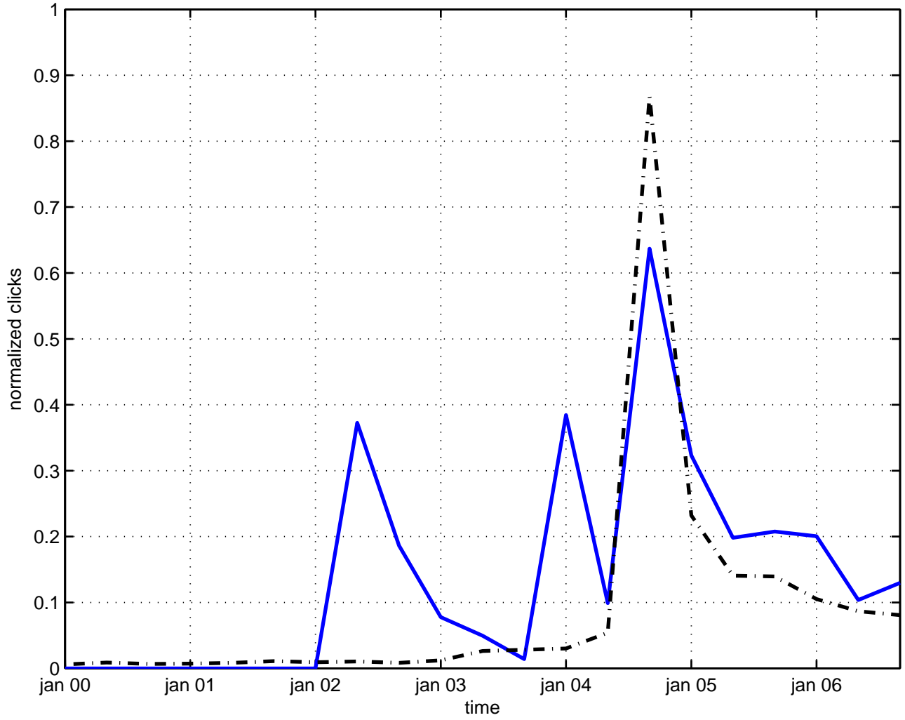
hard scattering
