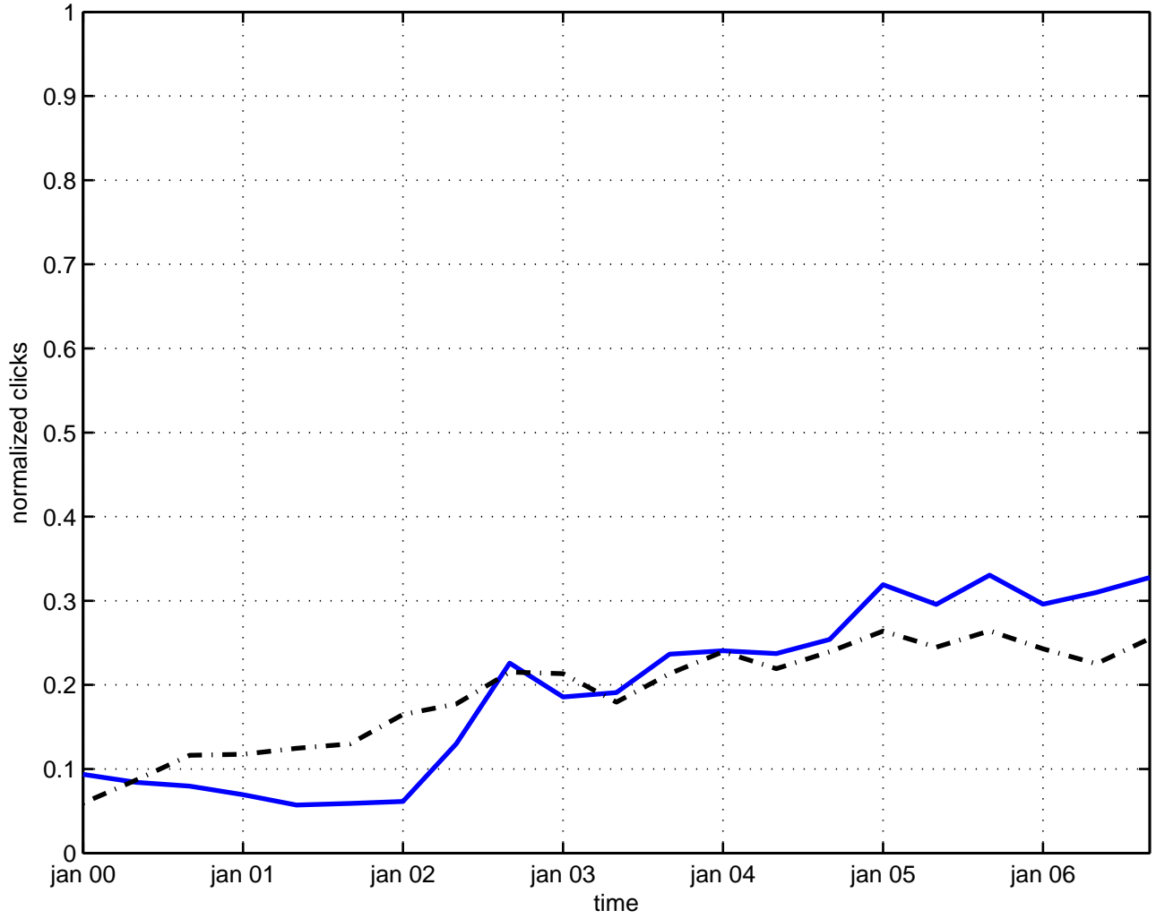
hamiltonian formalism
