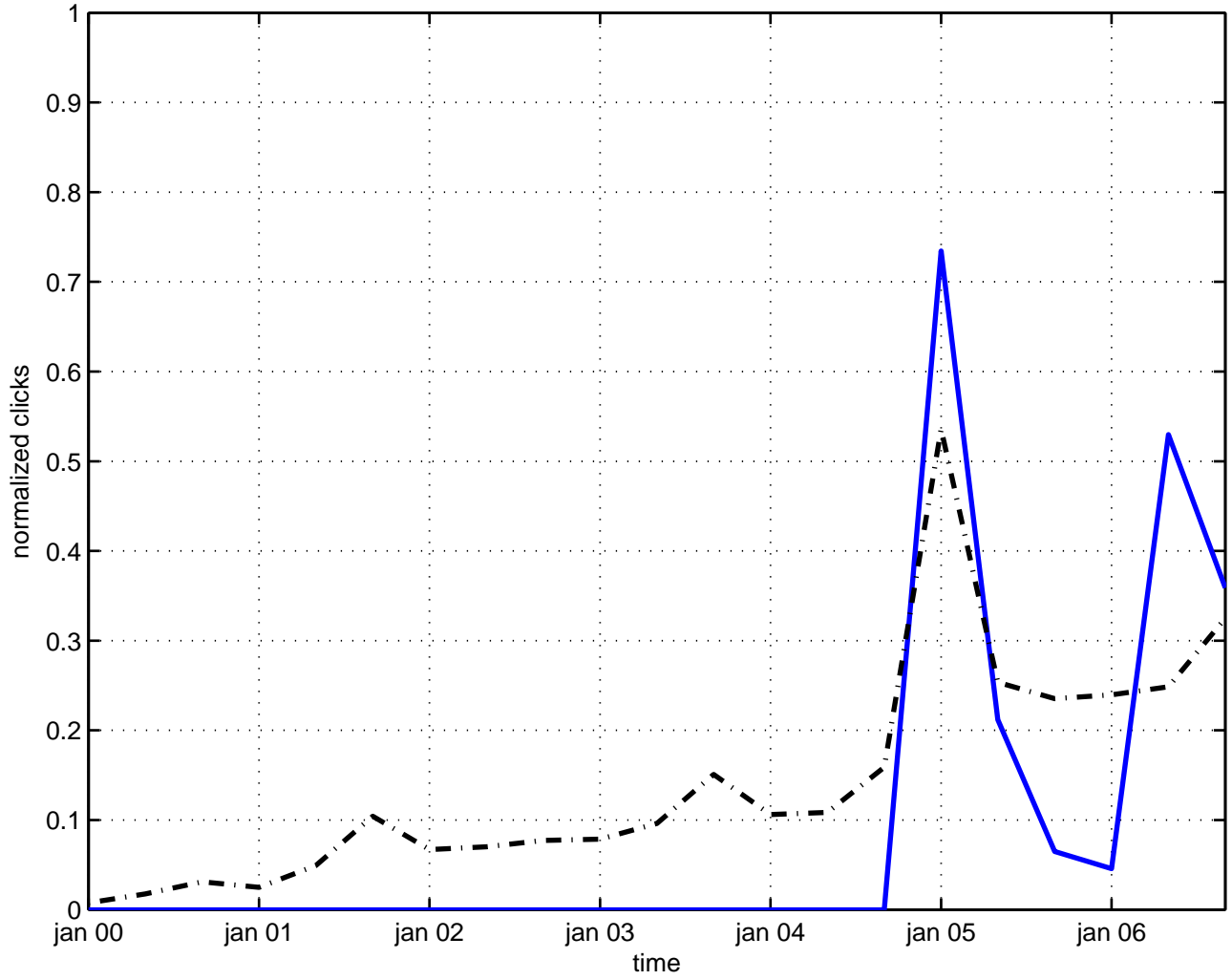
hadronic matter
