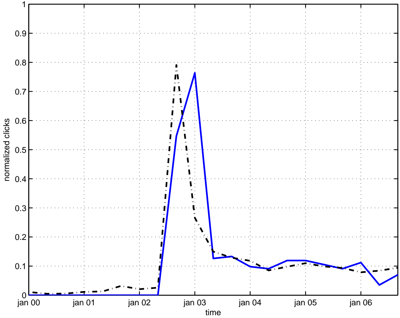
hadronic decay k0
