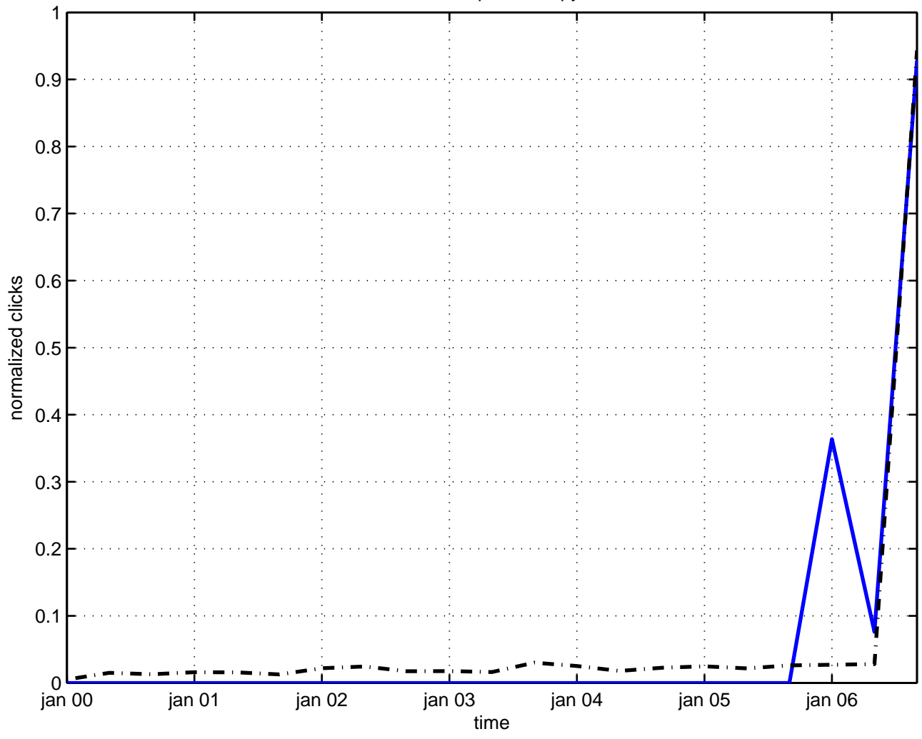
hadron spectroscopy
