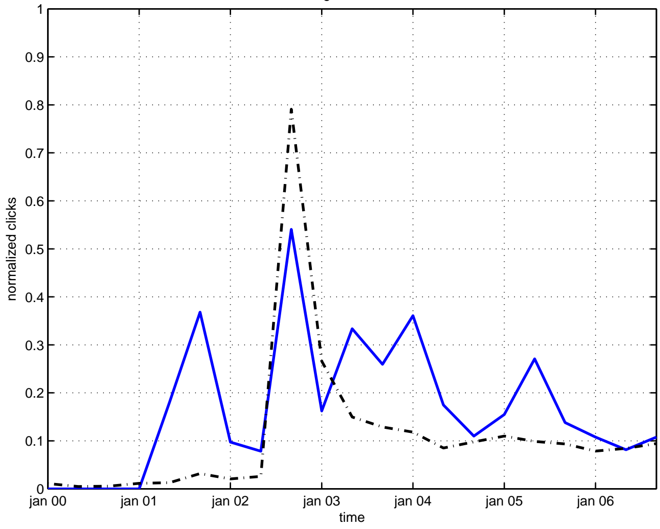
gzk effect
