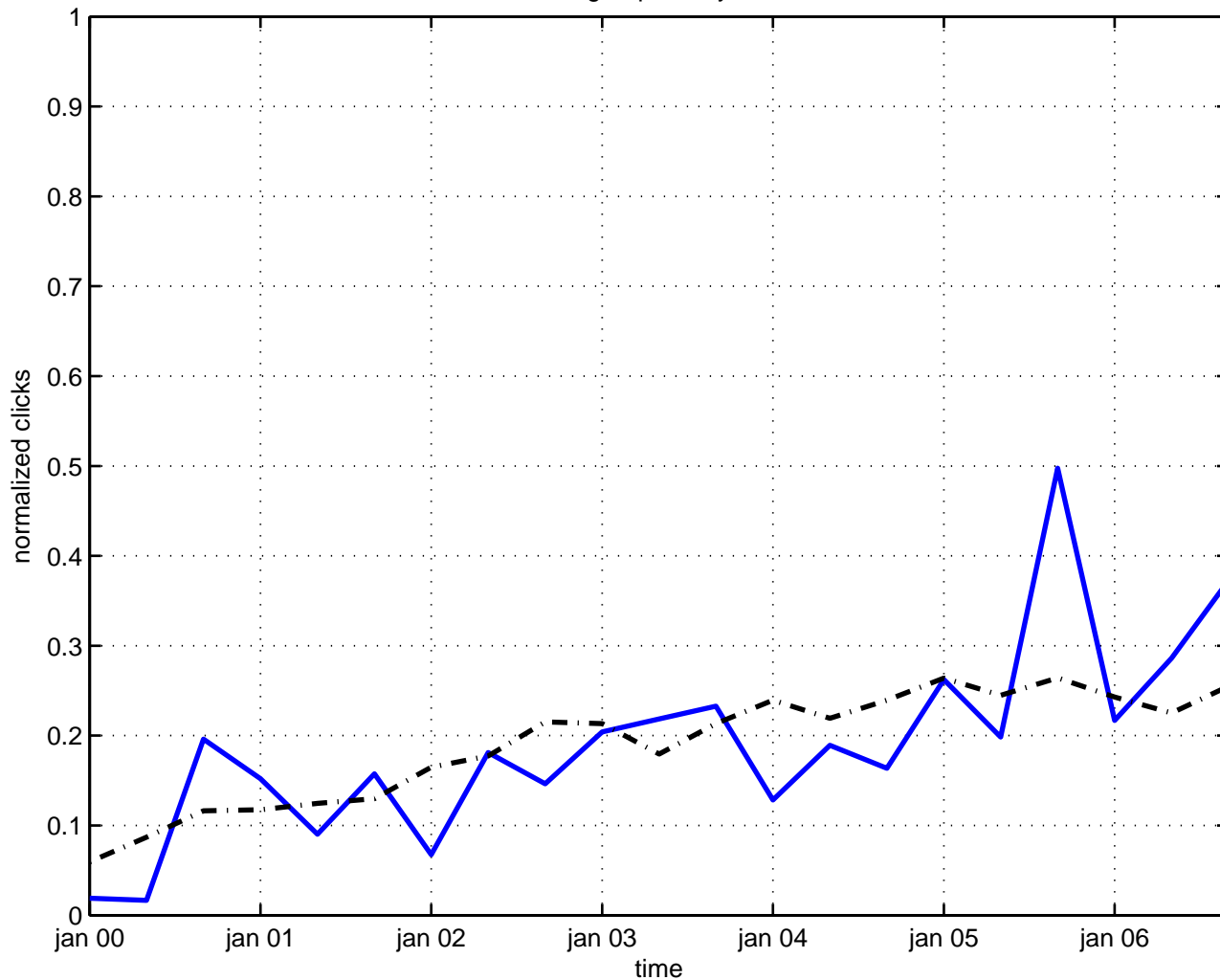
group theory
