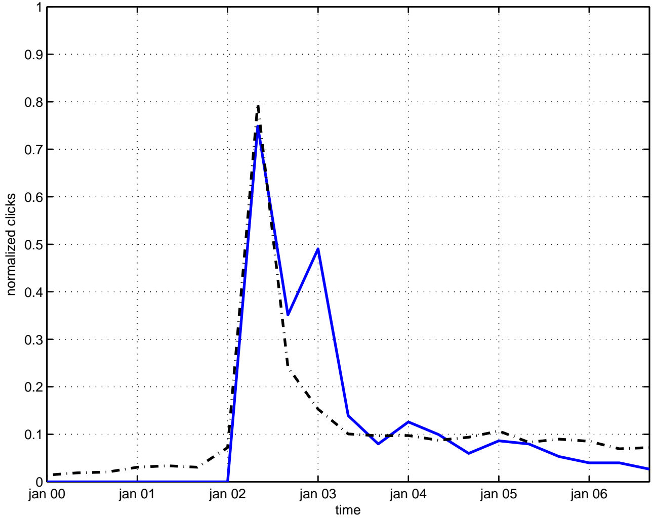
ground state black hole
