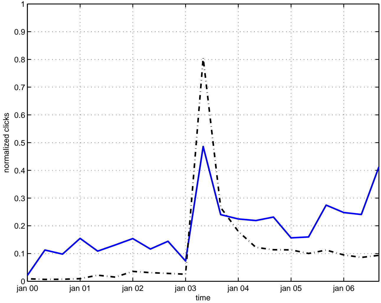
gross-neveu model
