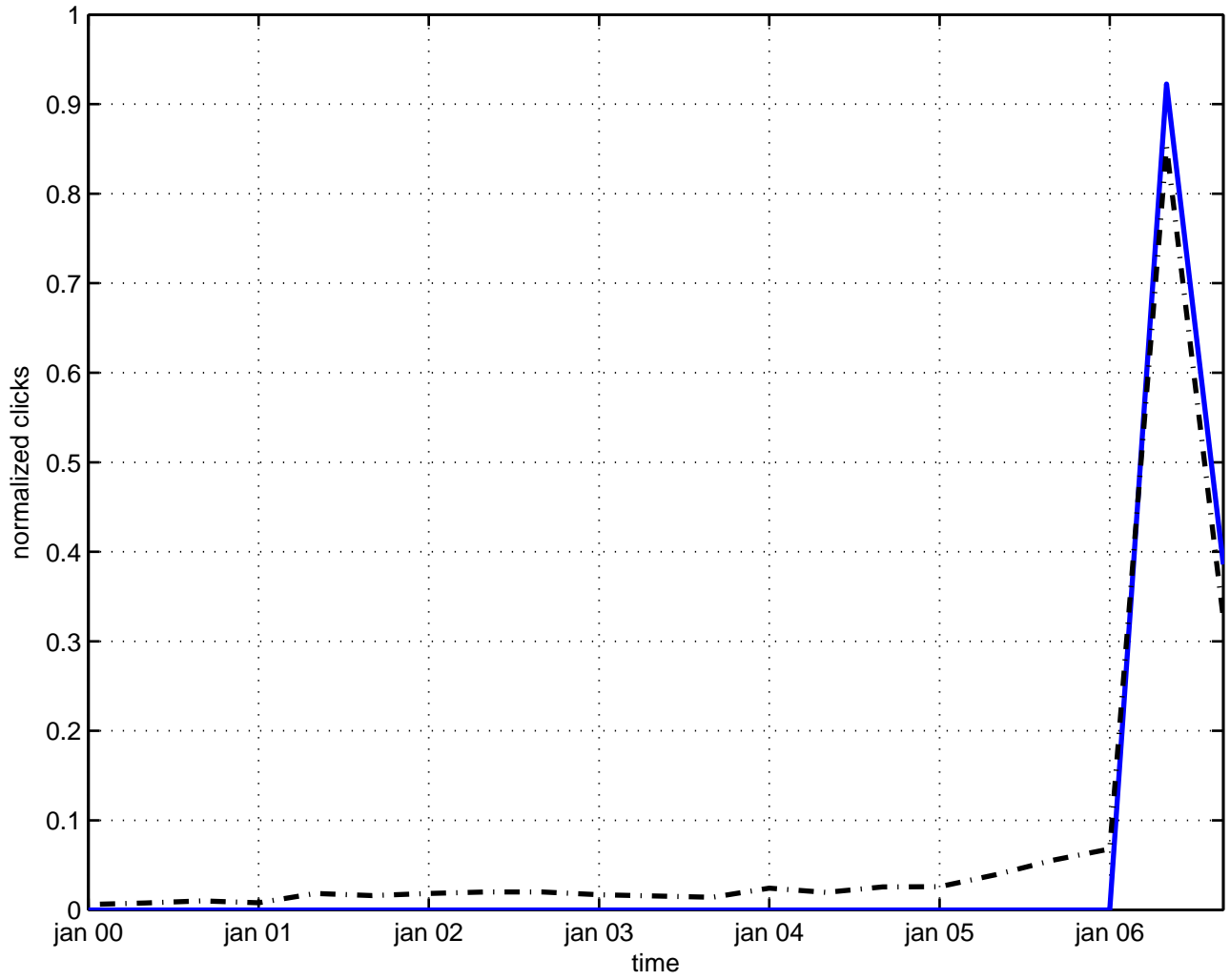
gravitation dyon
