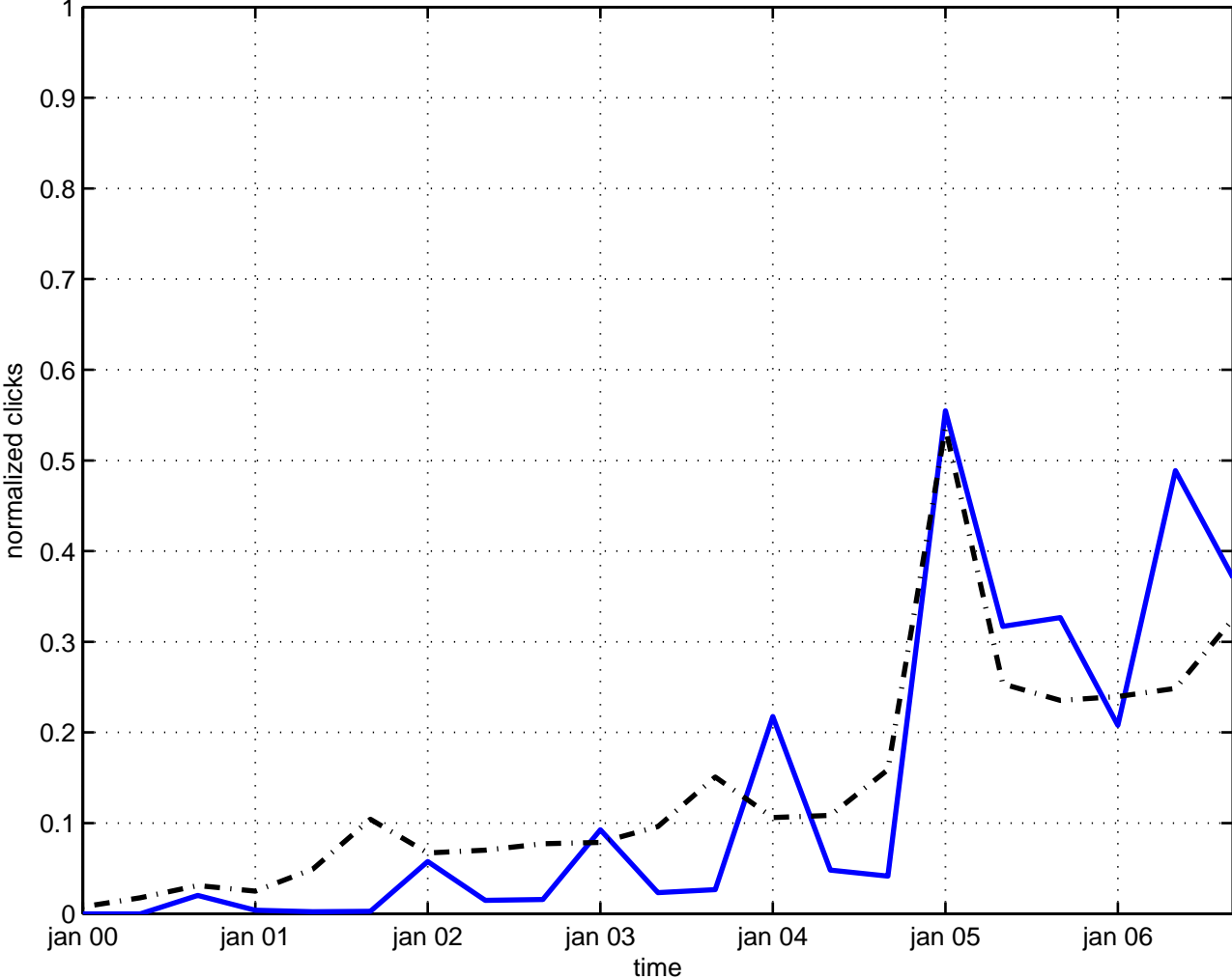
gravitation anomaly
