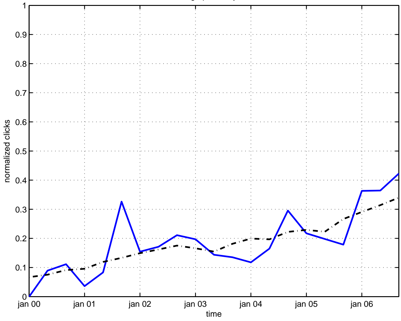
graph theory
