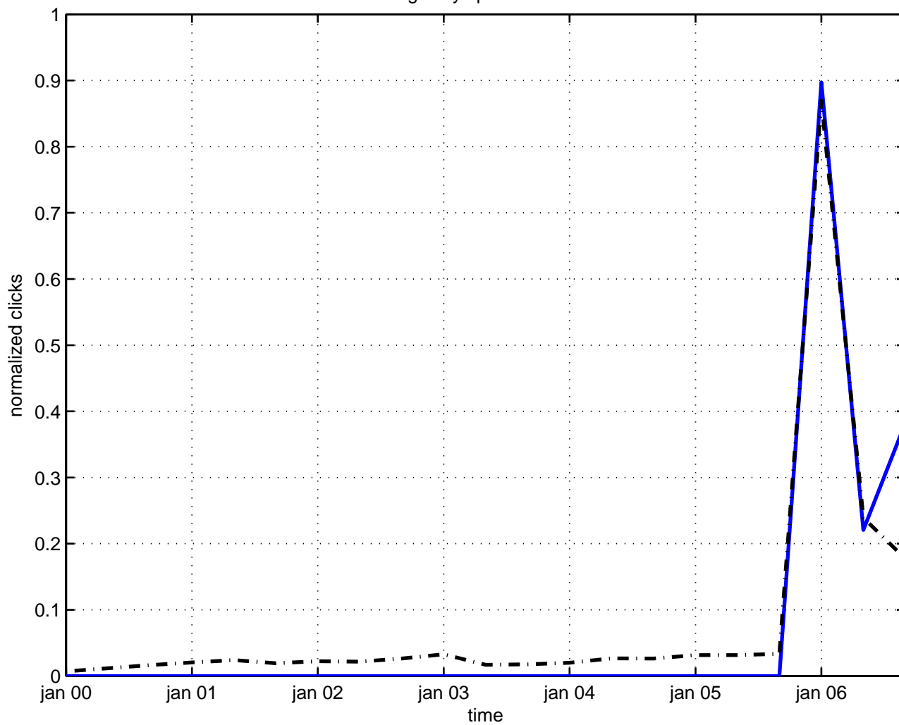
gowdy space-time
