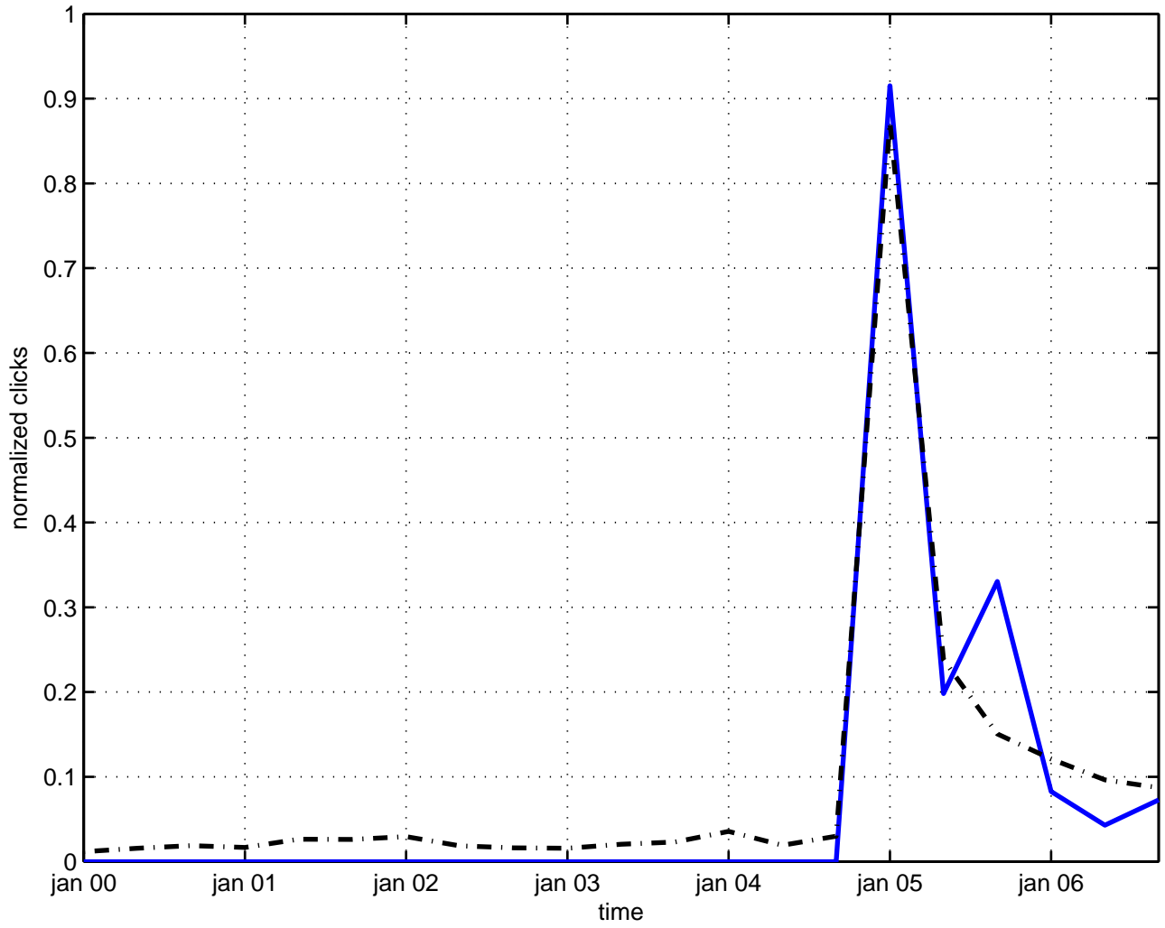
gott space-time
