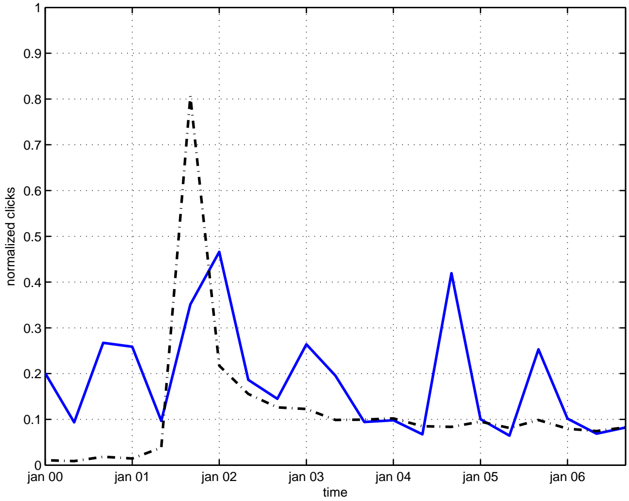
goldstone theorem
