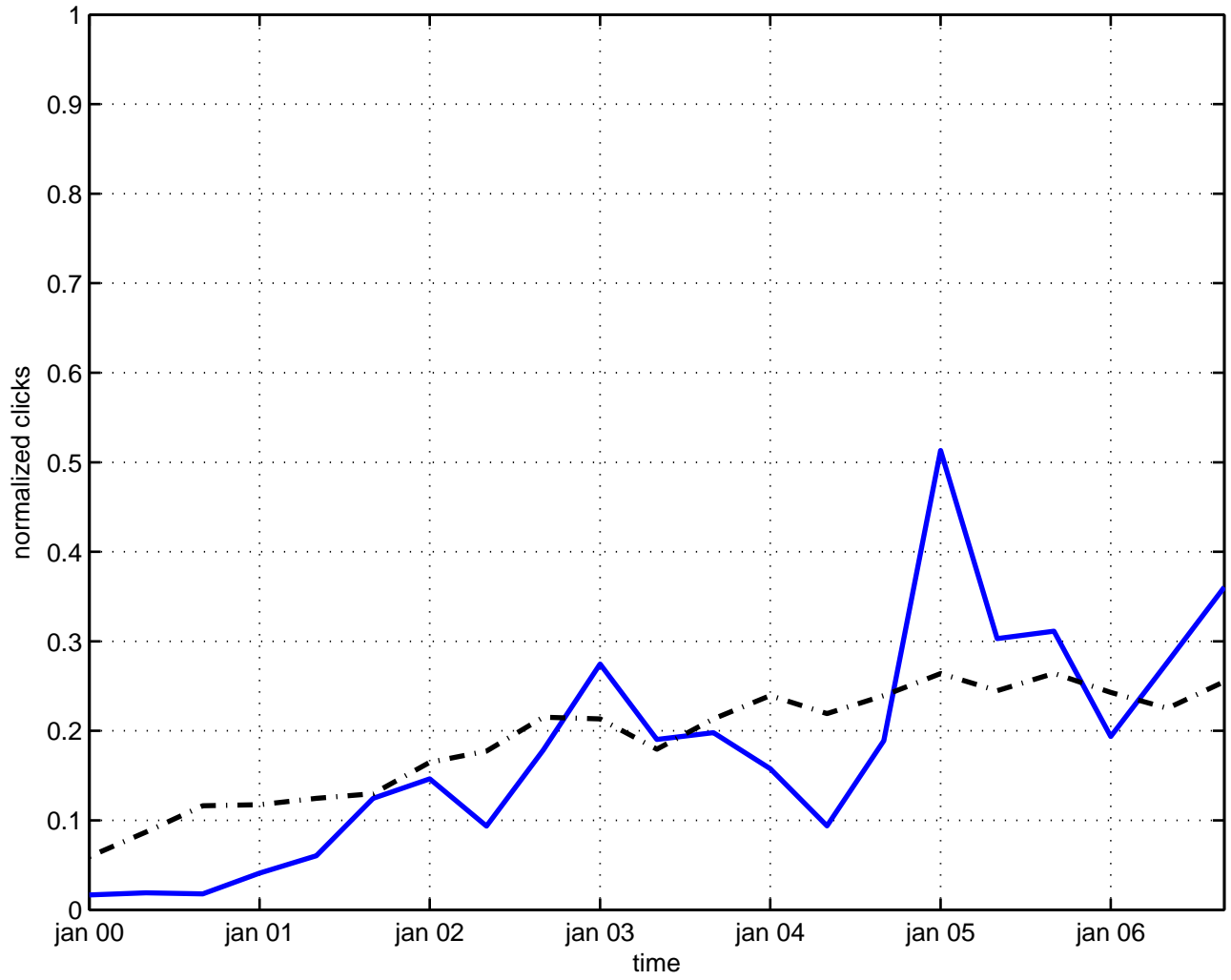
goldstone particle
