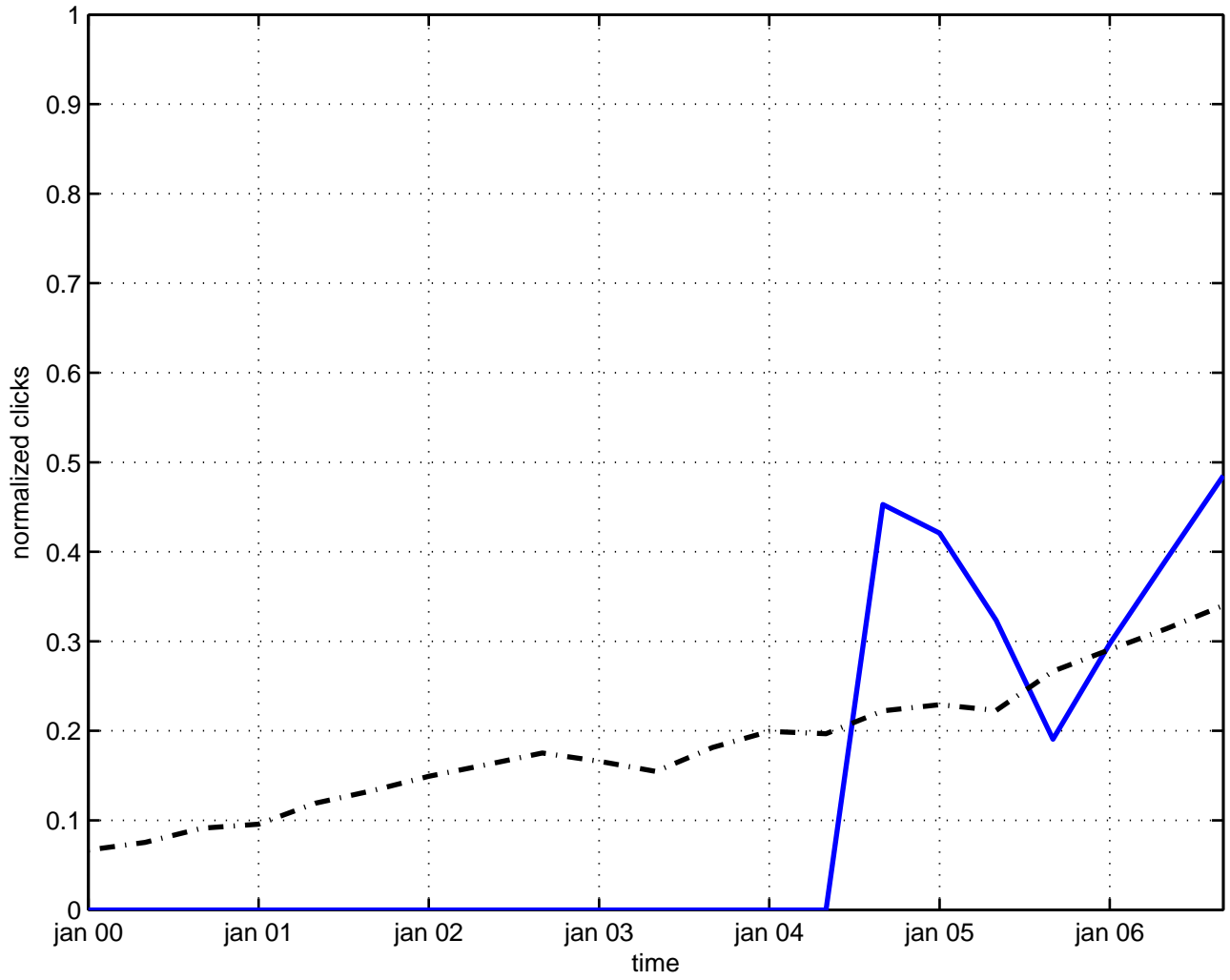
goldstone particle pi
