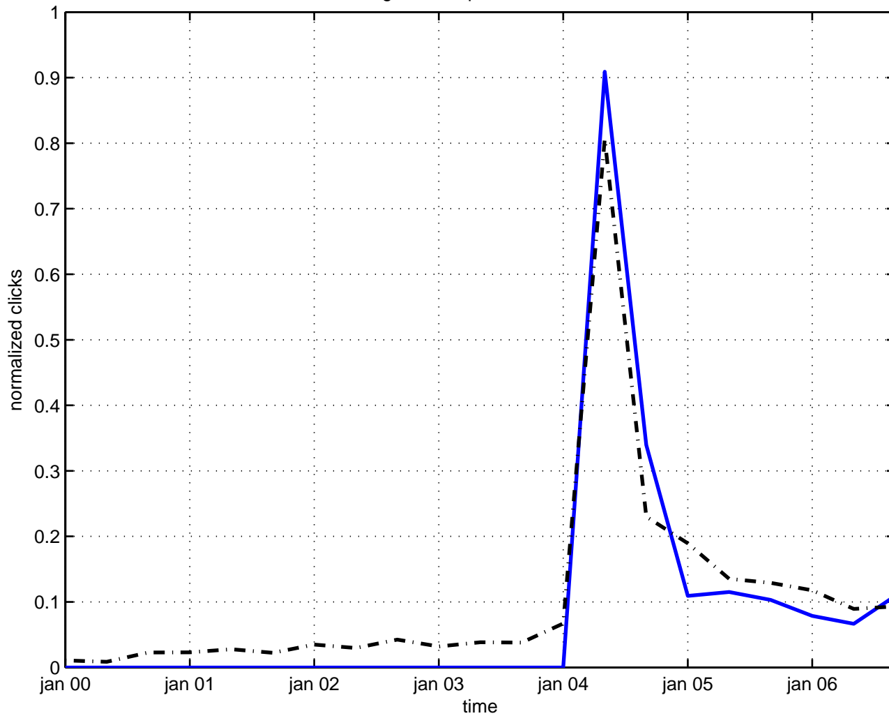
goldstone particle axion
