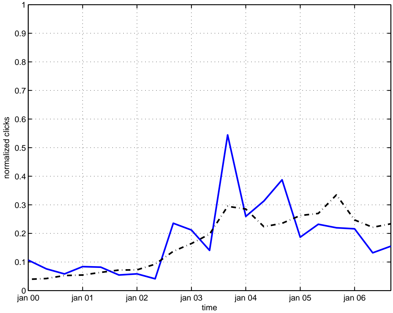
glueball
