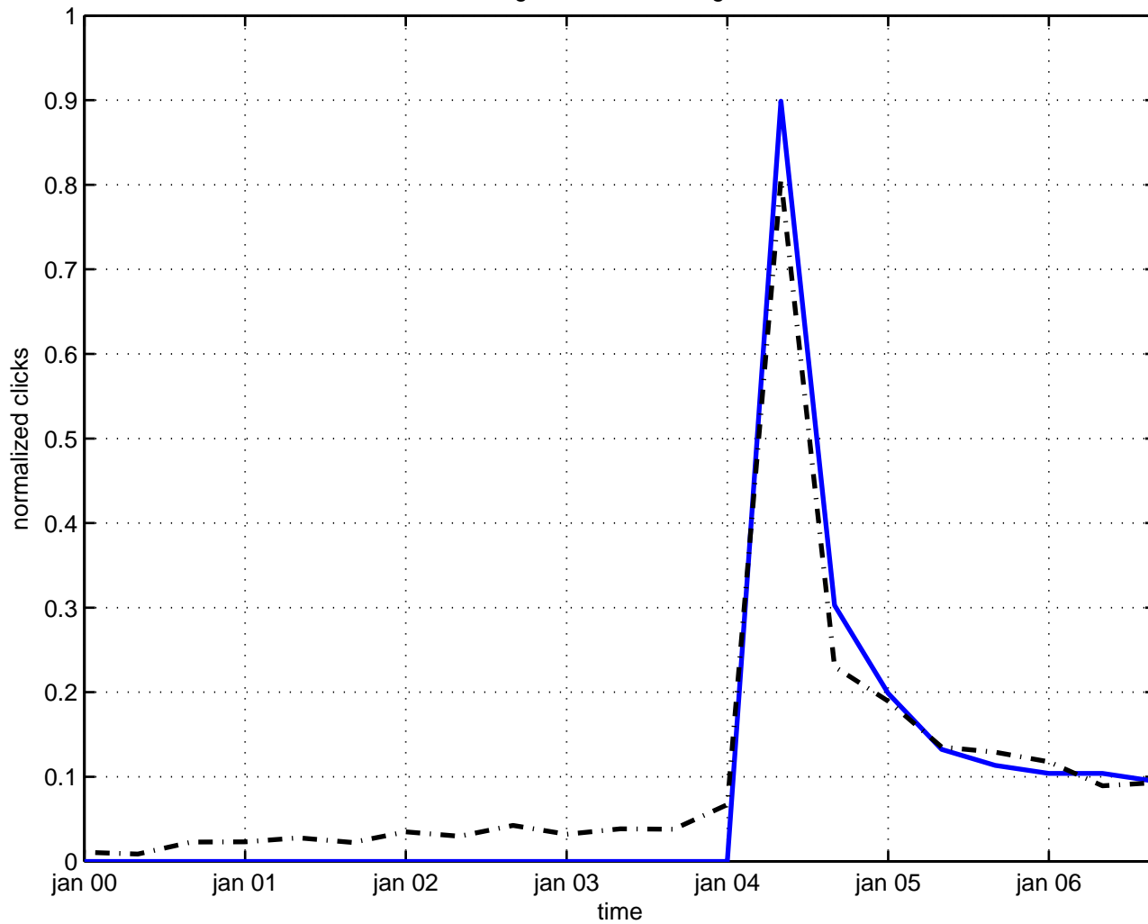
global cosmic string
