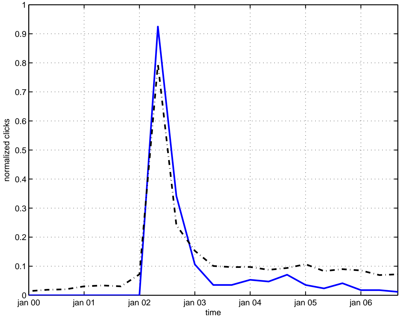
glashow algebra
