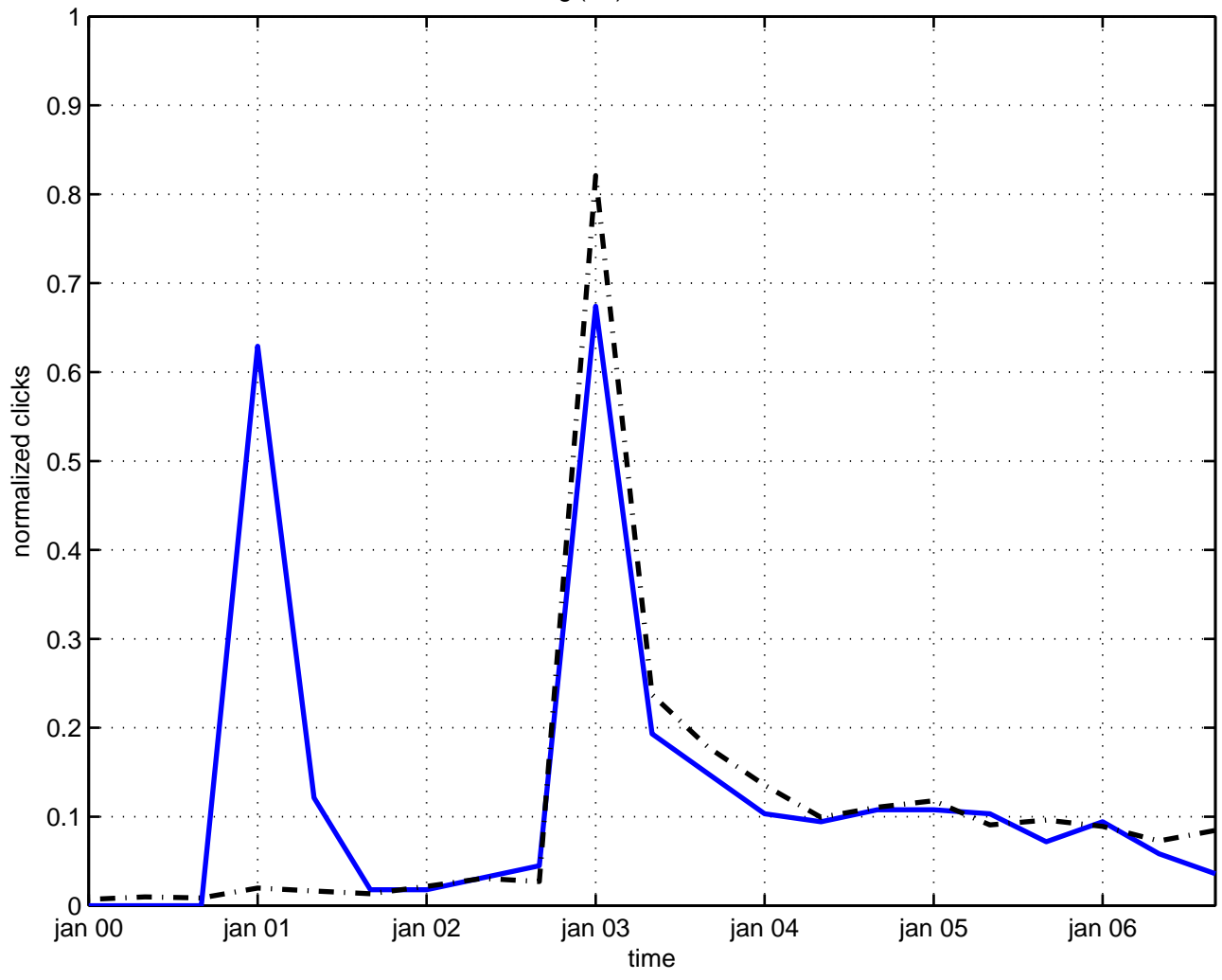
gl(n,r) invariance
