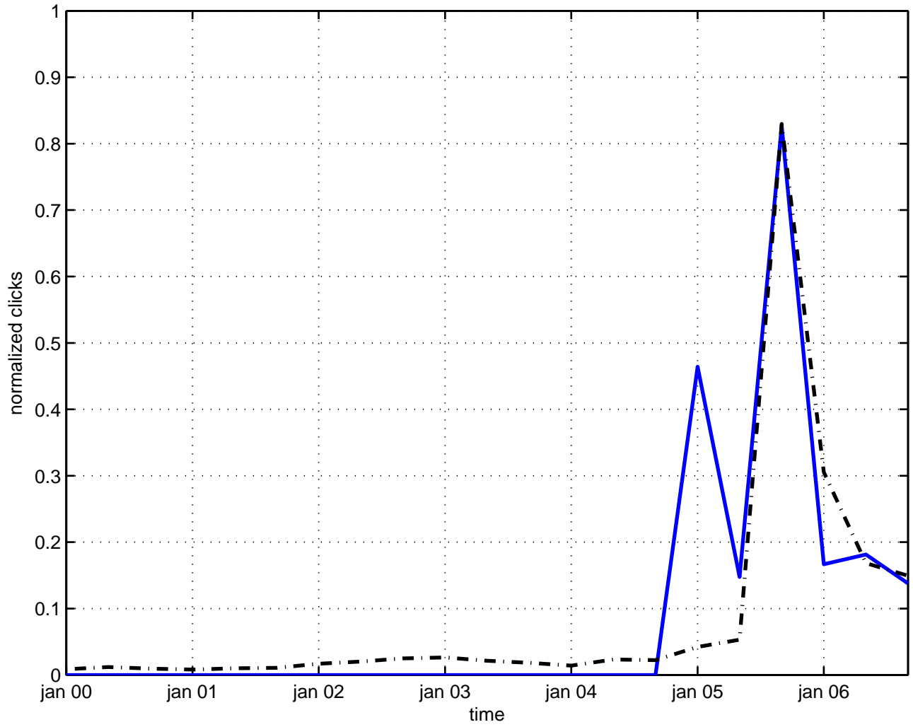
gl(n) symmetry
