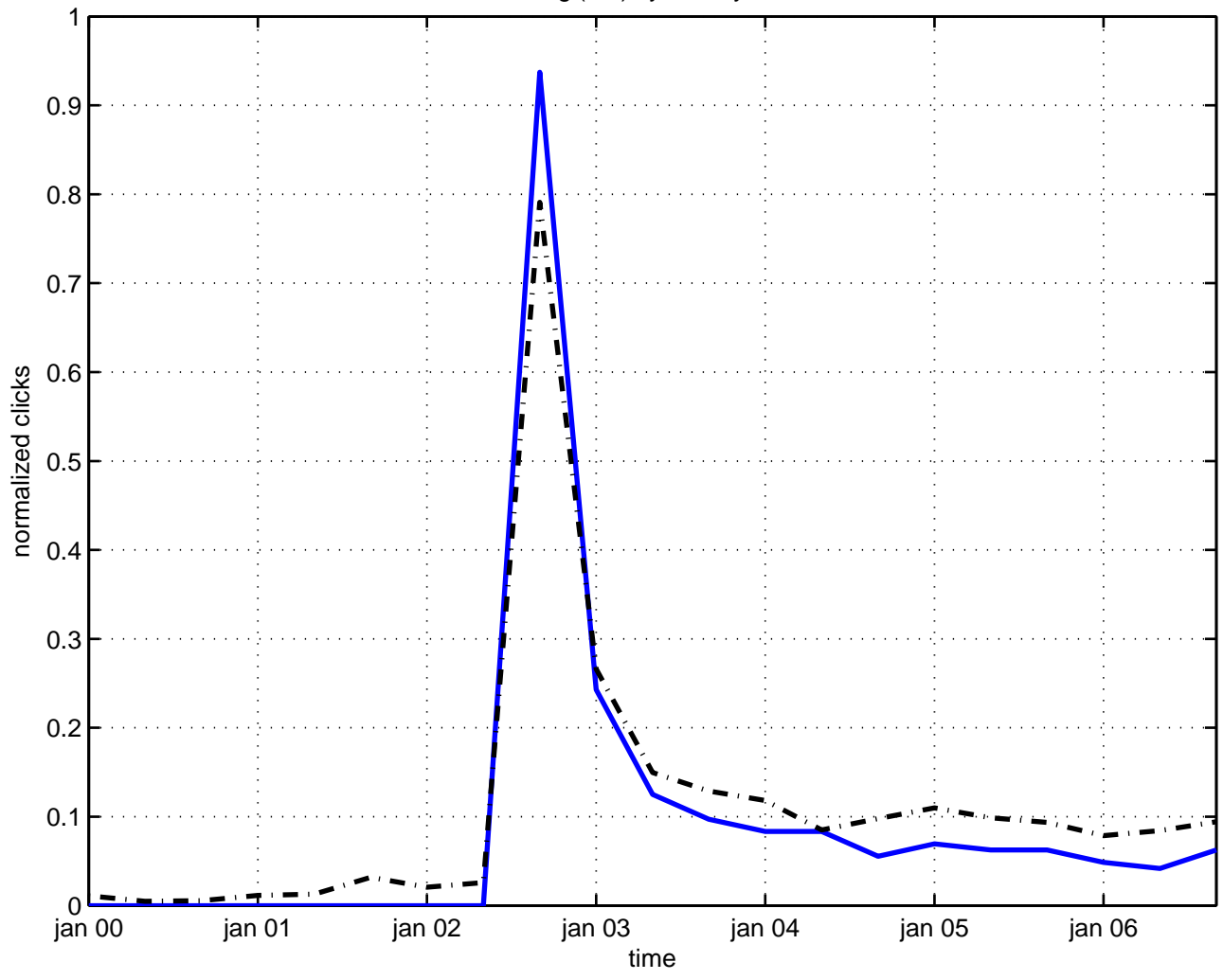
gl(2/2) symmetry
