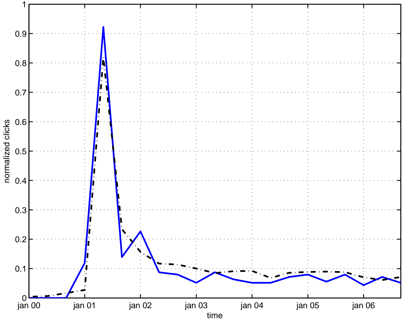
gl(2,c) gauge field theory
