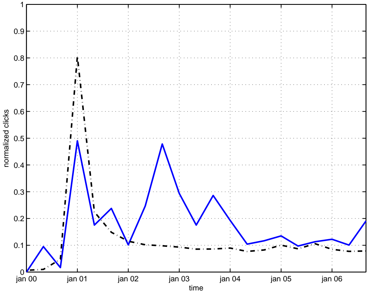
ginsparg-wilson relation
