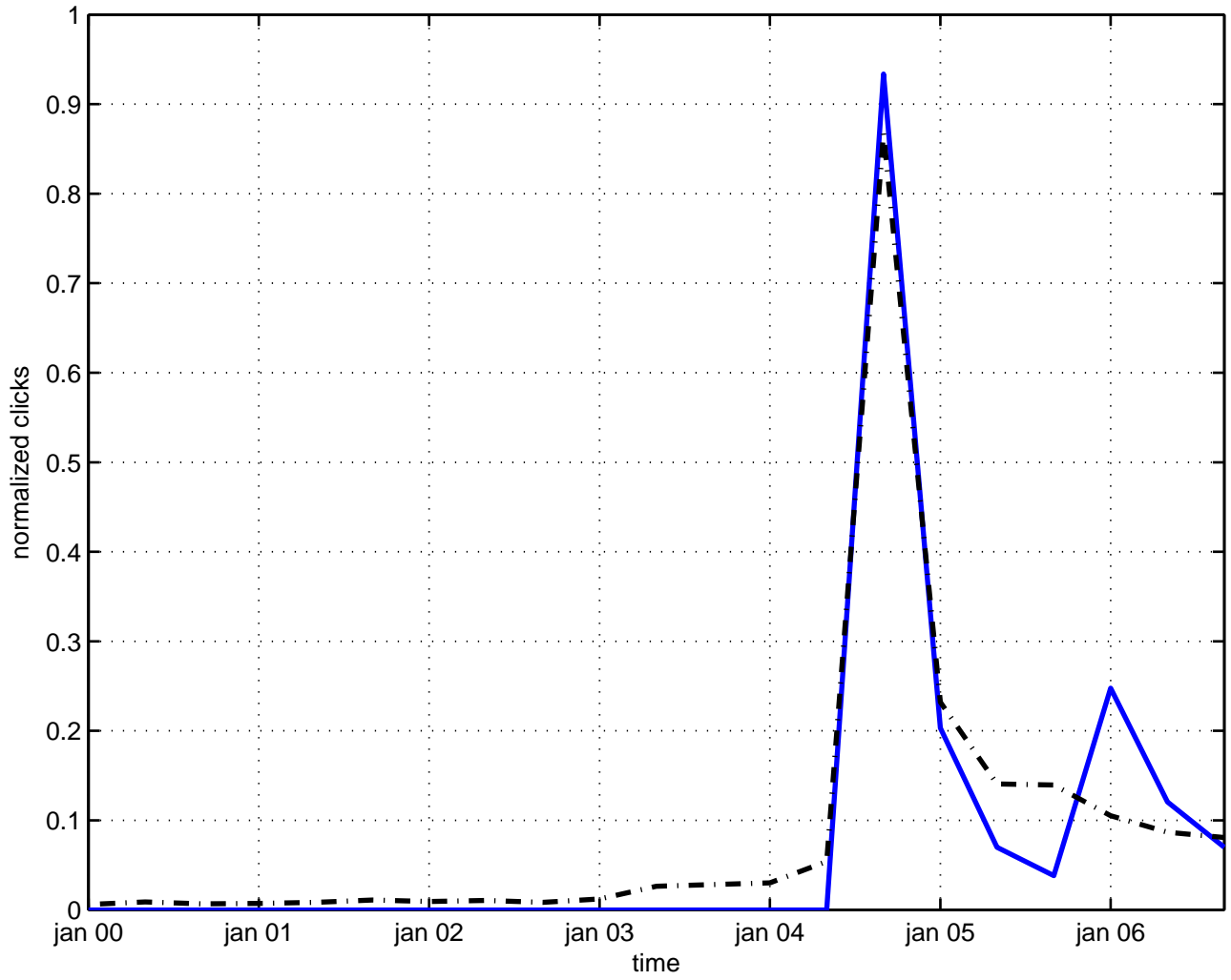
gibbons-maeda black hole
