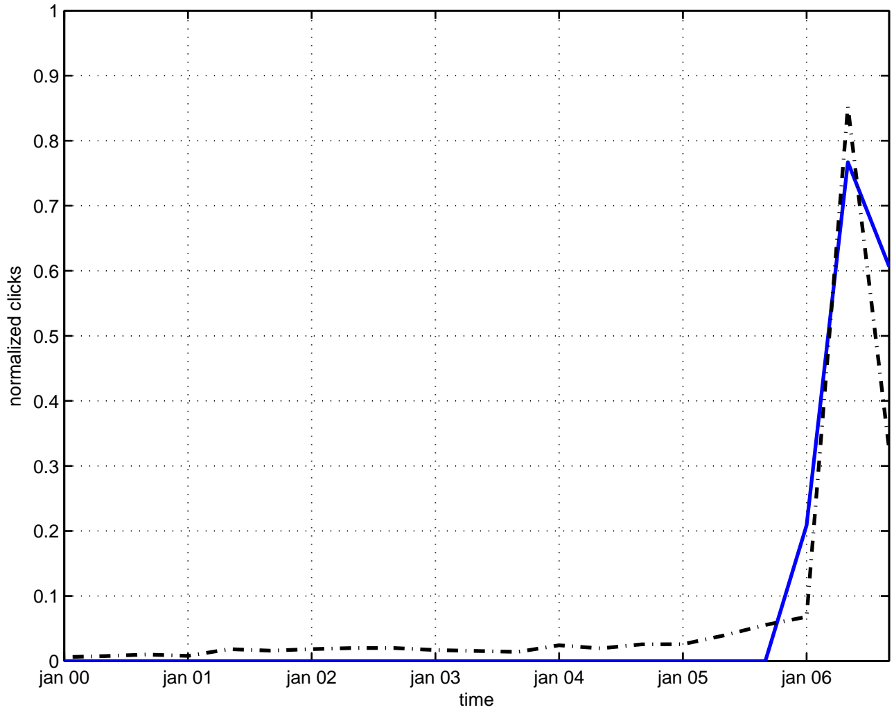
giant magnon
