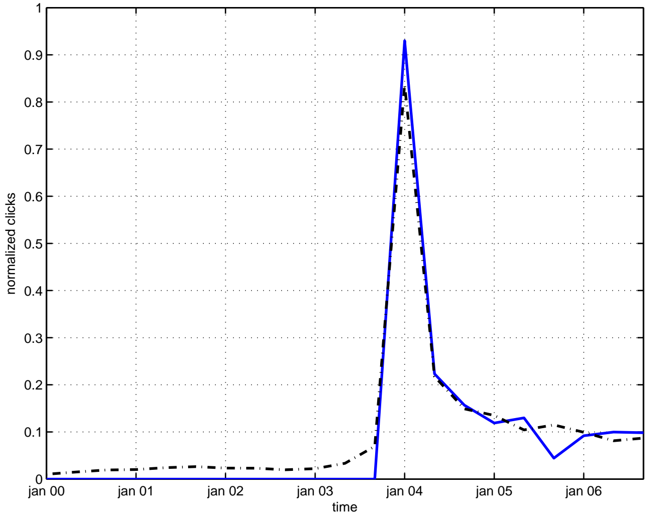
giant inflaton
