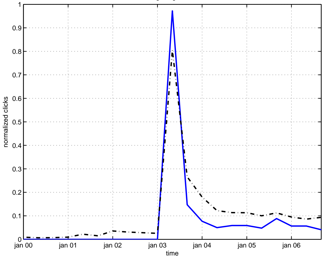
giant gluon
