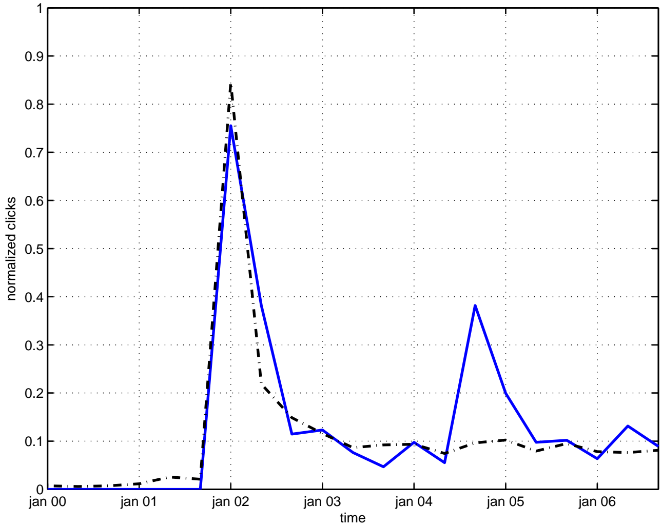
gerstenhaber algebra
