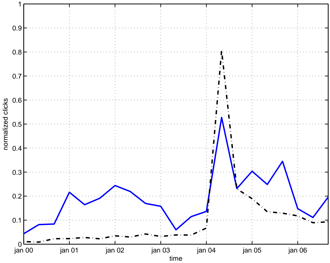
georgi-glashow model
