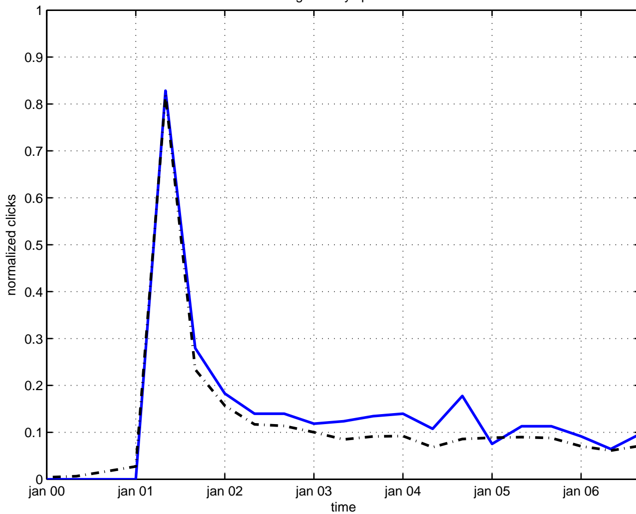
geometry spinor
