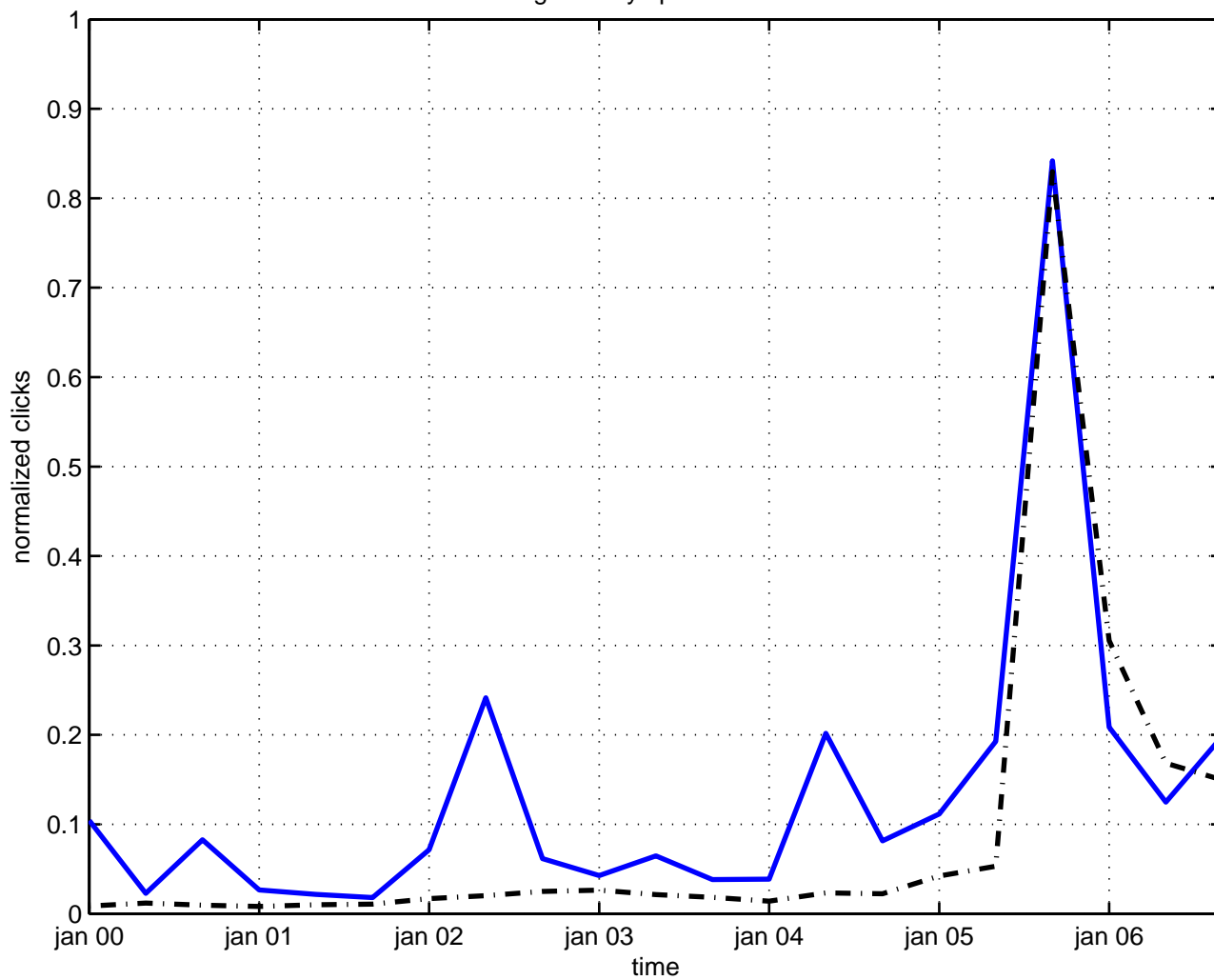
geometry space-time
