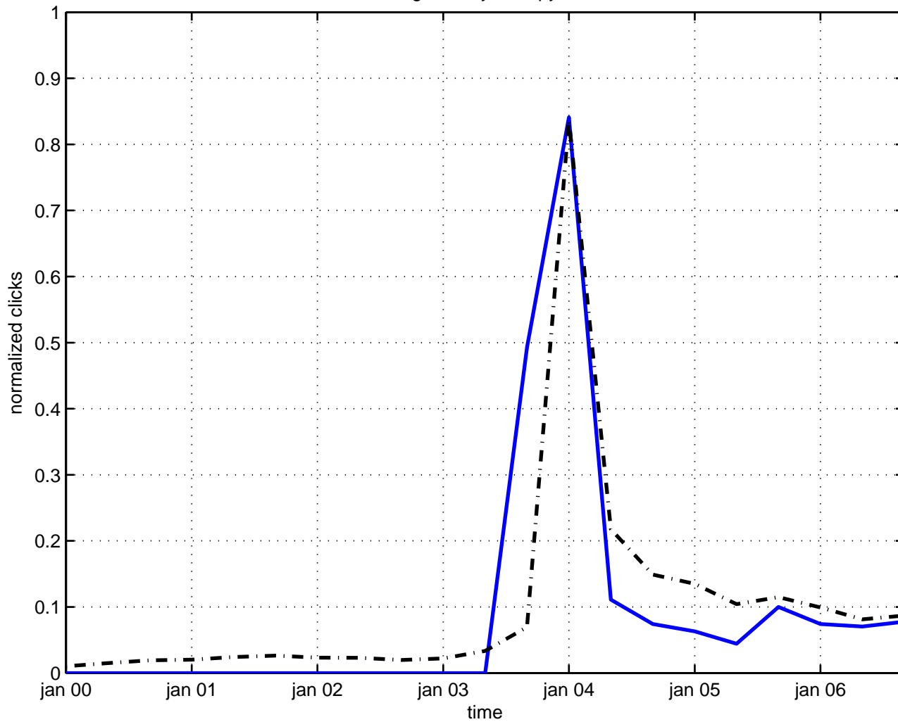
geometry entropy
